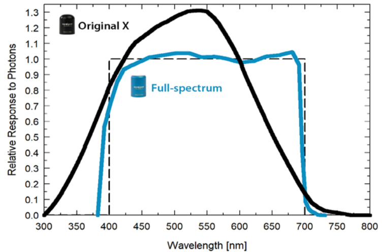
Mean spectral response measurements of six replicate Apogee MQ-210X and MQ-510 series quantum sensors.
