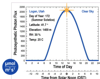
MODEL FOR QUANTUM SENSOR PHOTOSYNTHETIC PHOTON FLUX
