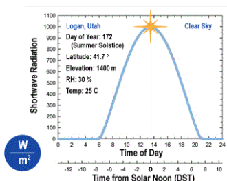
MODEL FOR PYRANOMETER SHORTWAVE RADIATION
