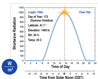
MODEL FOR PYRANOMETER
